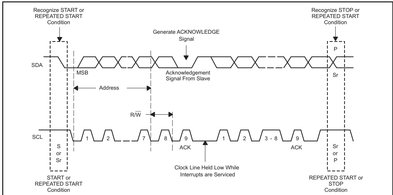
Figure 116. I²C Bus Protocol
