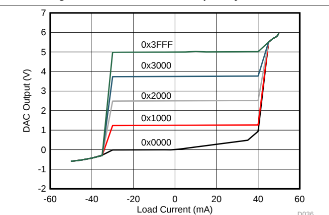
Figure 34. Source and Sink Capability with Gain = 1/2
