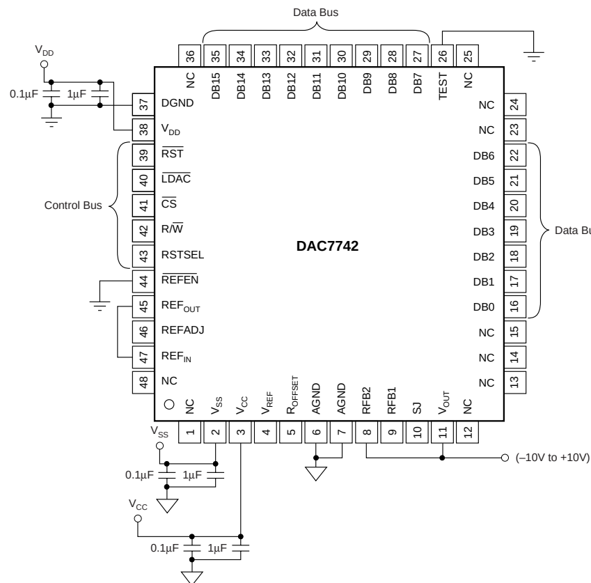
FIGURE 4. Basic Operation: V_{OUT} = -10V to +10V .
