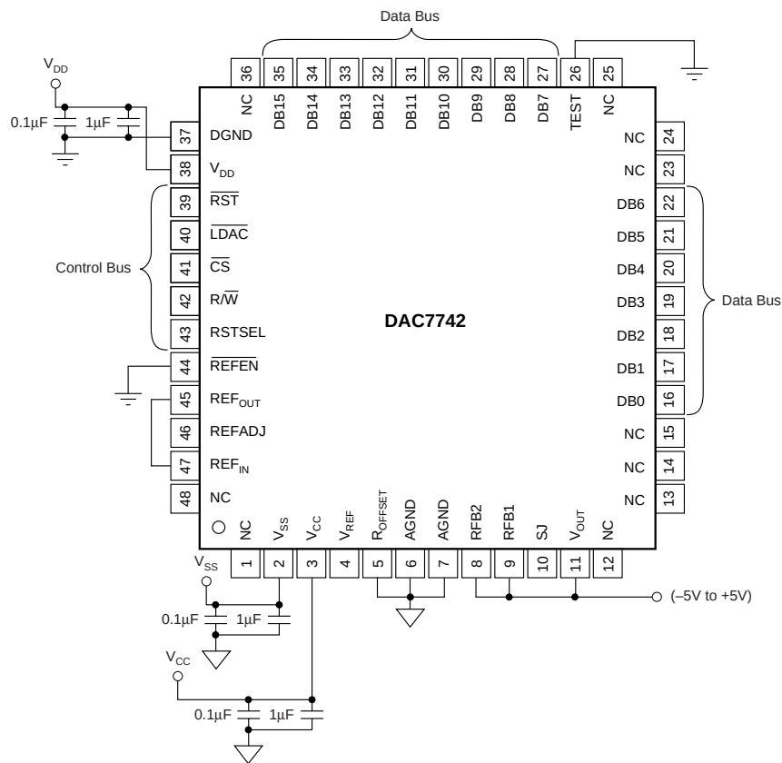
FIGURE 3. Basic Operation: V_{OUT} = -5V to +5V .
