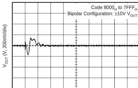
MID-SCALE GLITCH
