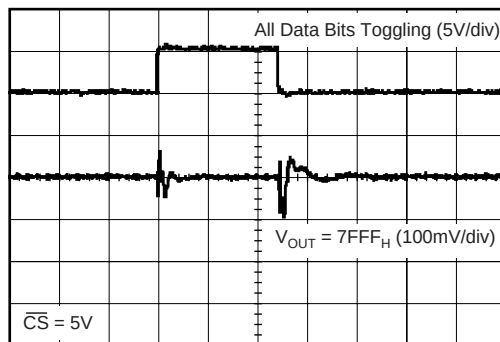
DIGITAL FEEDTHROUGH
