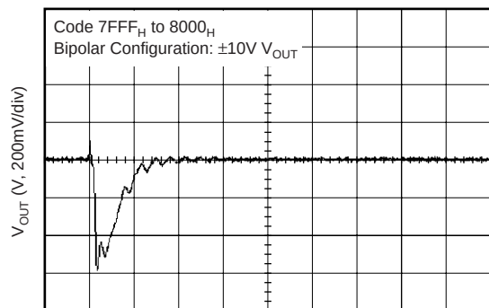
MID-SCALE GLITCH
