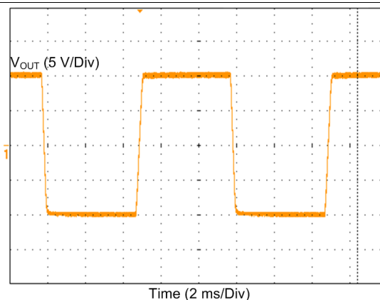
Figure 77. Full-Scale Step Response
