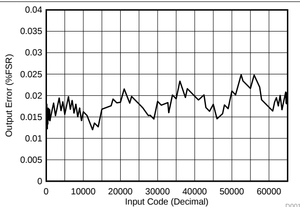
Figure 76. Output Voltage Error vs Input Code
