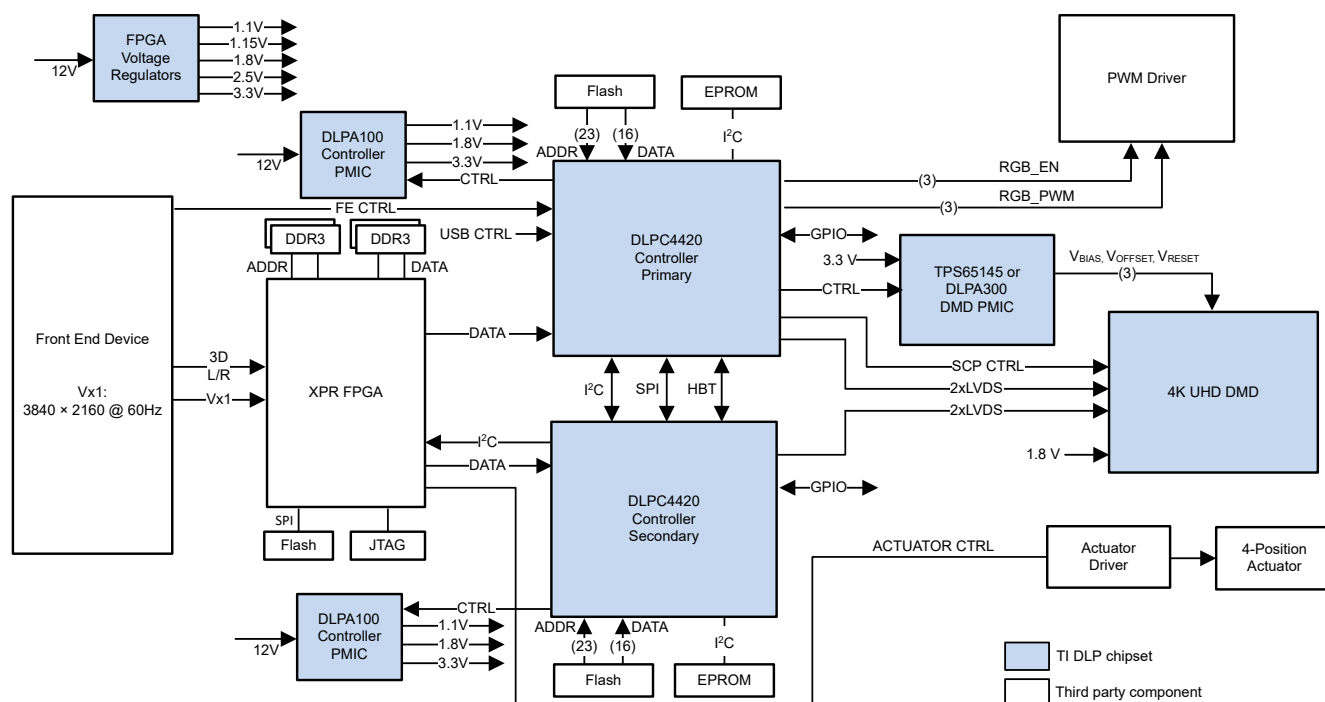
图 8-1. Typical 4K UHD LED Display Application
