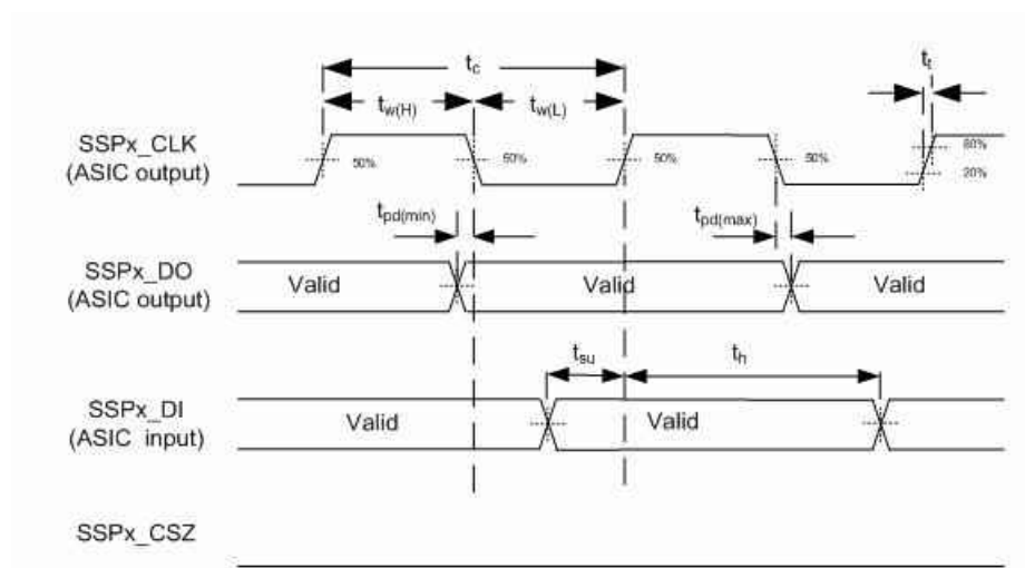
图 6-8. Synchronous Serial Port Interface - Secondary
