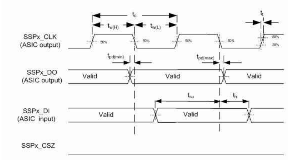
图 6-7. Synchronous Serial Port Interface - Primary
