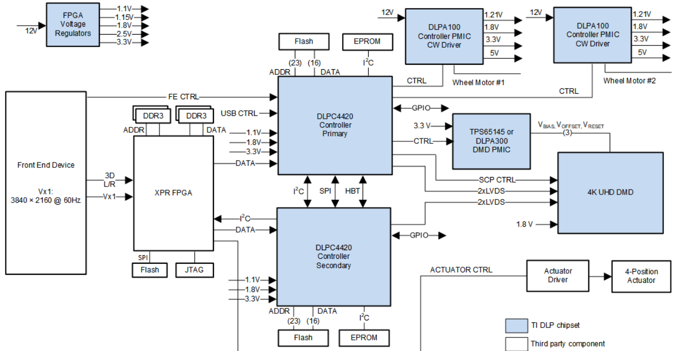
图 8-2. Typical 4K UHD LPCW Display Application
