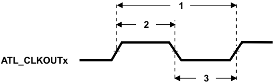
Figure 8-4. ATL_CLKOUTx Timing
