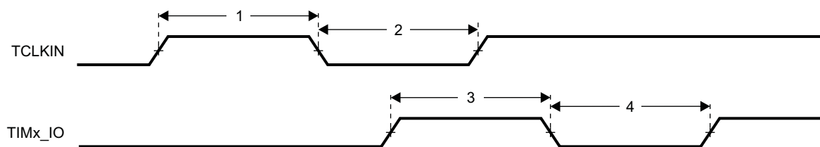
Figure 8-93. Timer Timing
