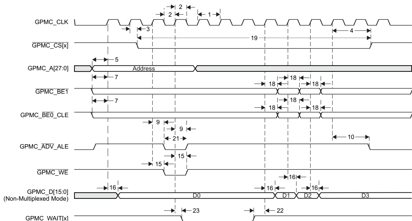
Figure 8-23. GPMC Non-Multiplexed NOR Flash - Synchronous Burst Write (GPMCFCLKDIVIDER = 0)
