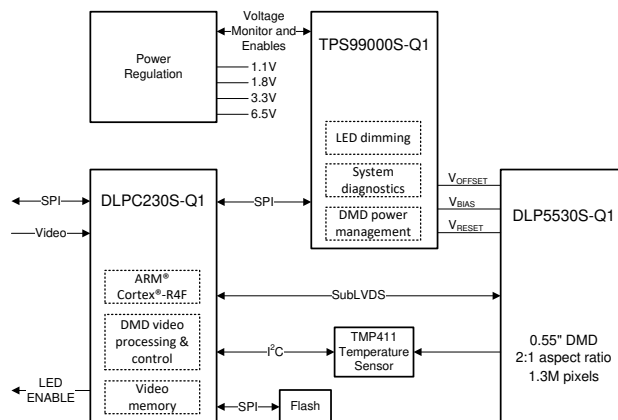
DLP553x-Q1 TI DLP® Chipset System Block Diagram
