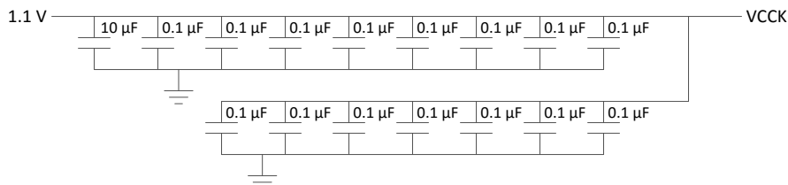
Figure 10-1. VCKK Recommended Filter
