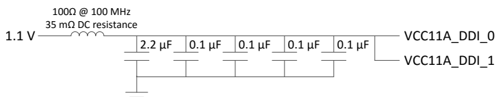
Figure 10-3. VCC11A_DDI Recommended Filter
