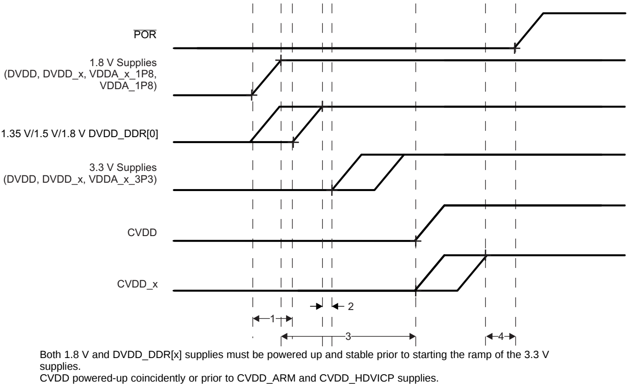
Figure 7-1. Power-Up Sequence
