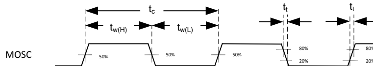
Figure 1. System Oscillators
