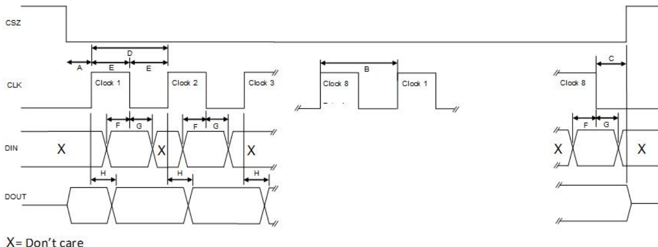
Figure 4. Serial Communications Port Timing Diagram
