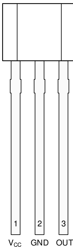
图 5-2. LPG Package 3-Pin TO-92 Top View
