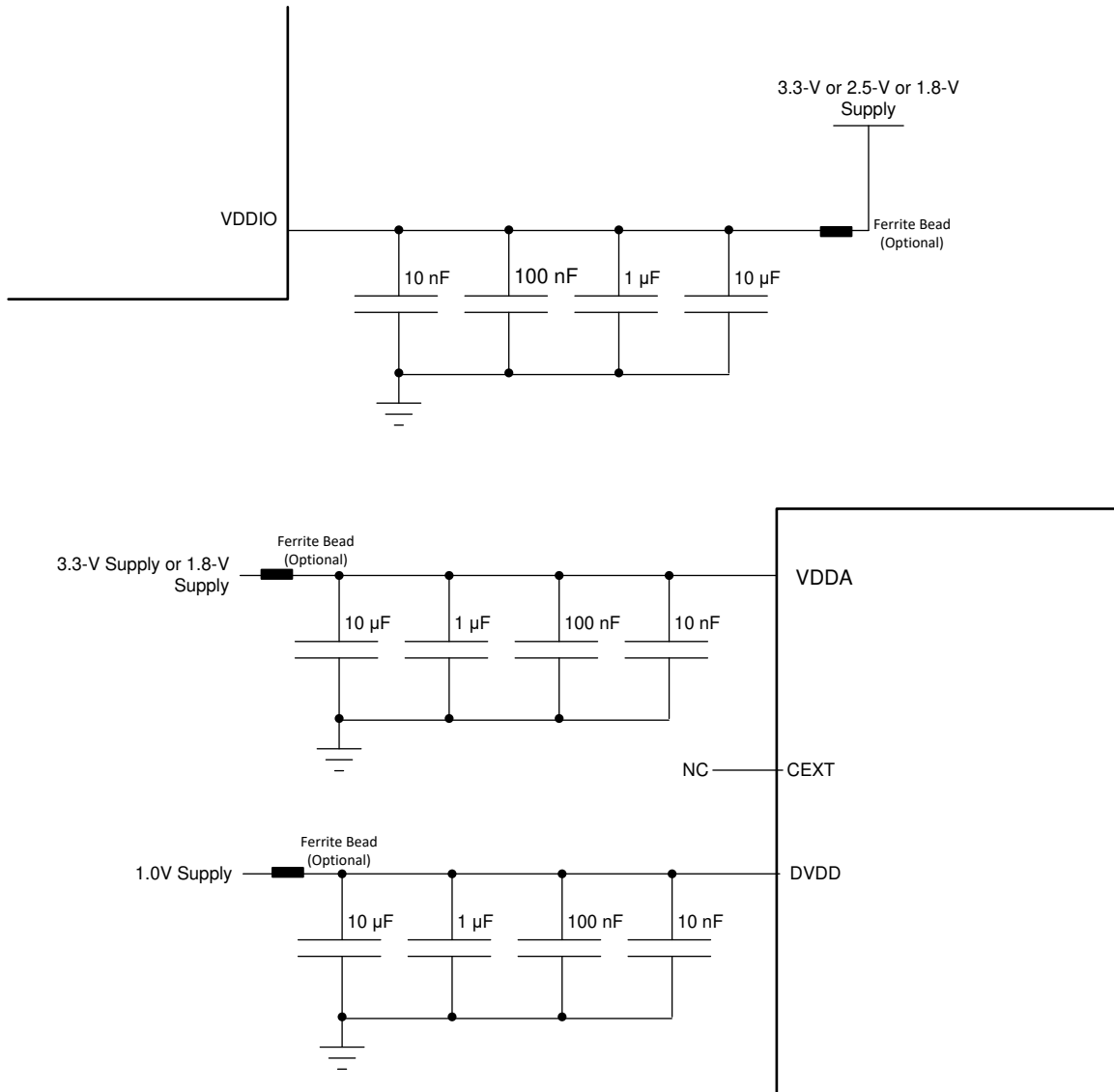
图 9-2. DP83TD510E Dual Supply Power Supply Decoupling Recommendation
