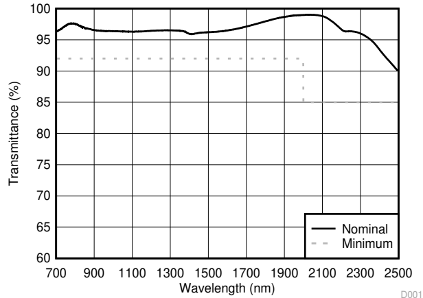
7-5. DLP4500NIR DMD Window Transmittance
