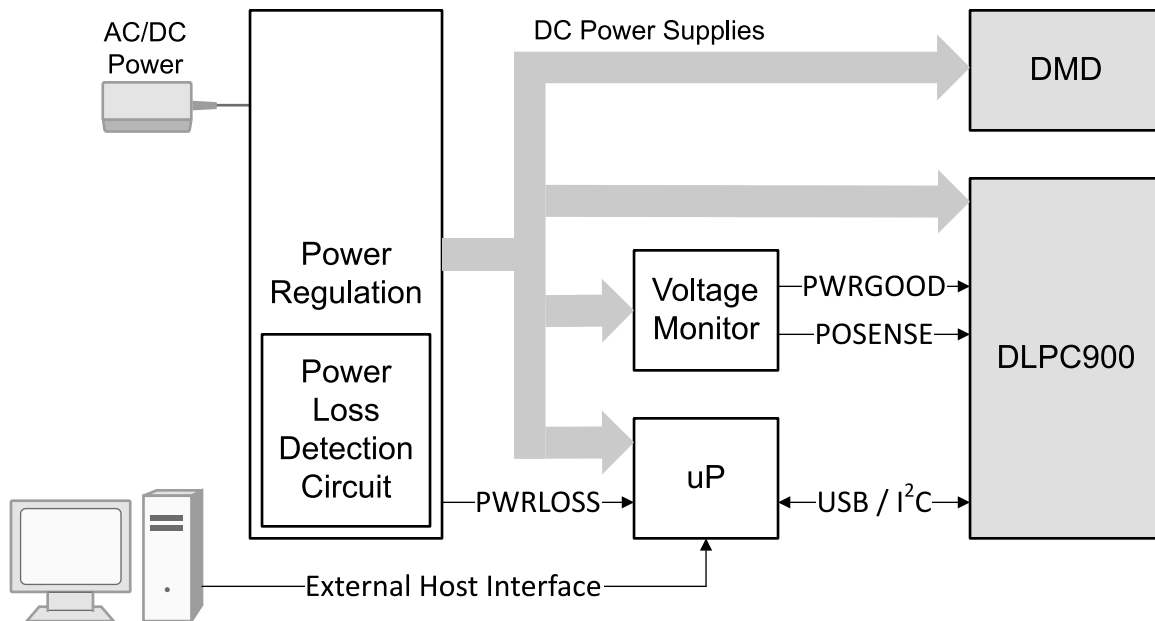
图 6-3. Power Distribution Layout Example
