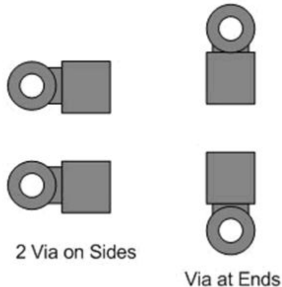
Figure 10-6. Decoupling Via Placement
