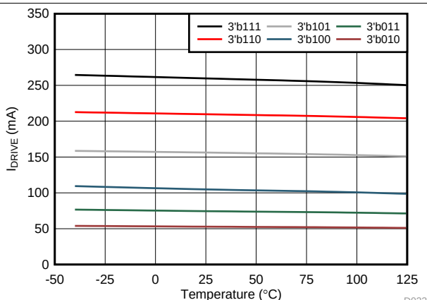
图 23. Low-Side Source Current
