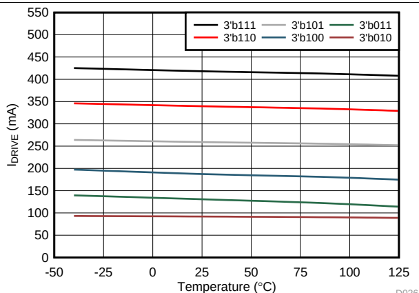
图 26. High-Side Sink Current
