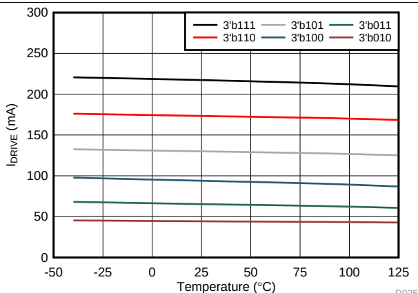
图 25. High-Side Source Current
