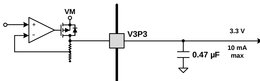
Figure 21. LDO Diagram
