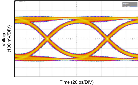
Figure 9. Typical Output Eye Diagram for the DS125RT410 Operating at 10.3125 Gbps With Default VOD of 600 mVp-p and De-emphasis Setting of –2 dB
