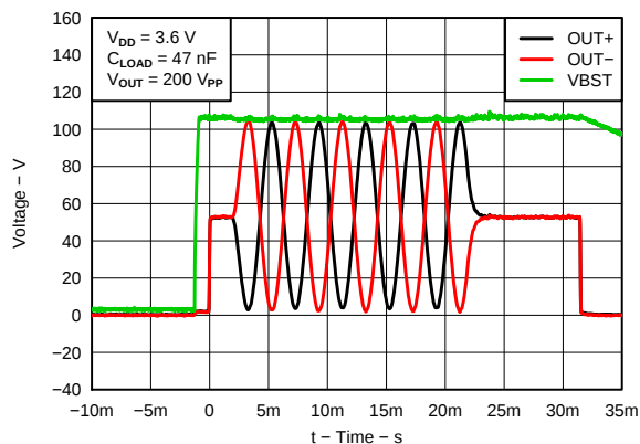
Figure 15. Typical Waveform
