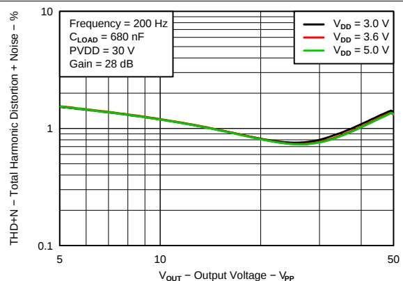
Figure 9. Total Harmonic Distortion + Noise vs Output Voltage
