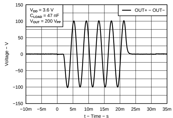
Figure 16. Typical Waveform - Differential
