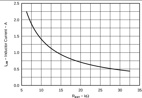
Figure 12. I_{LIM} vs R_{EXT}
