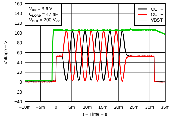
Figure 8. Typical Waveform
