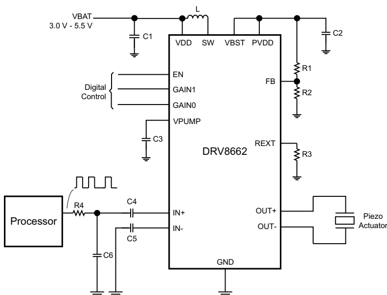
Figure 17. DRV8662 System Diagram with Filtered Single-Ended PWM Input
