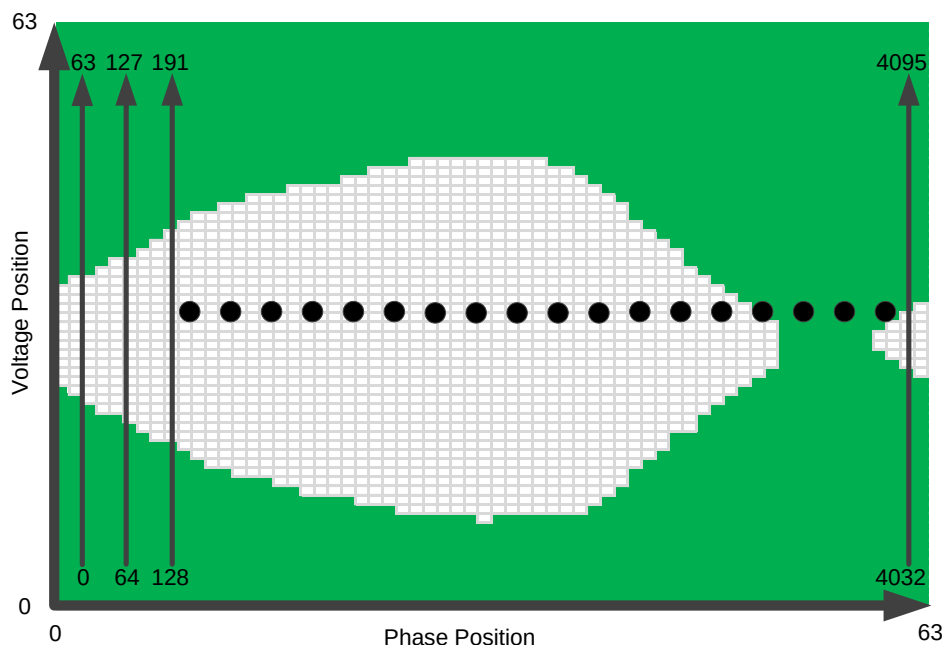
Figure 8. EOM Full Eye Capture Readout
