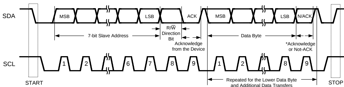
Figure 20. Basic Operation
