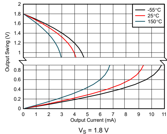
图 6-12. Output Voltage Swing vs. Output Current
