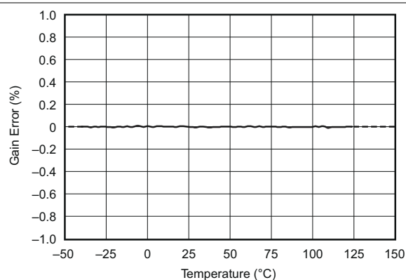
Figure 7-10. Gain Error vs. Temperature
