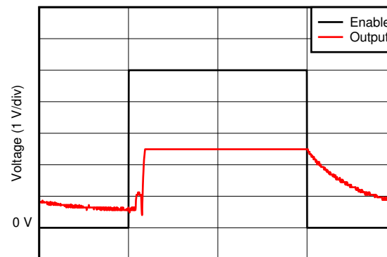
图 6-26. Start-Up Response
