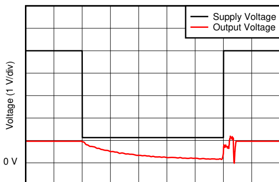
图 6-25. Noninverting Differential Input Overload
