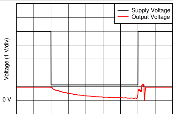
图 25. Noninverting Differential Input Overload
