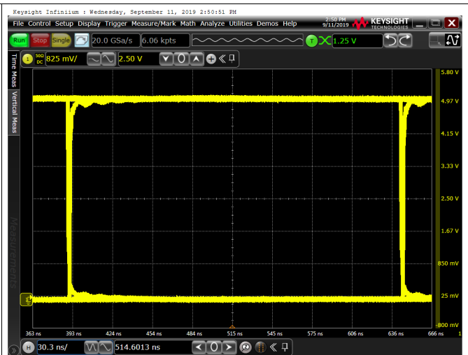
图 21. Eye Diagram at 4 Mbps PRBS 2^{16} - 1 , 5 V and 25°C
