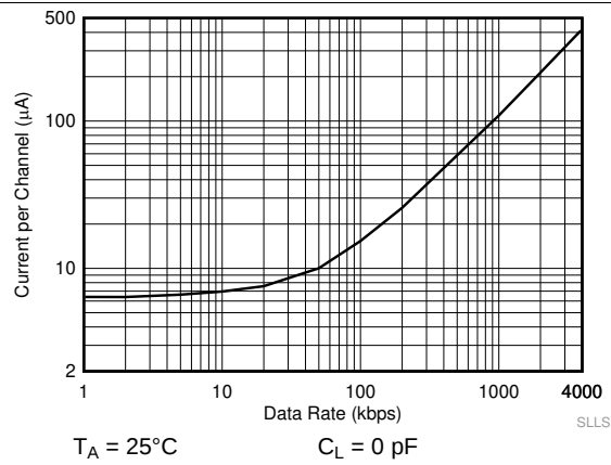
图 9. ISO7021 Supply Current vs Data Rate at 5 V (With No Load)
