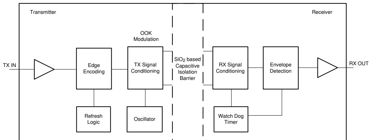
图 14. Conceptual Block Diagram of a Digital Capacitive Isolator
