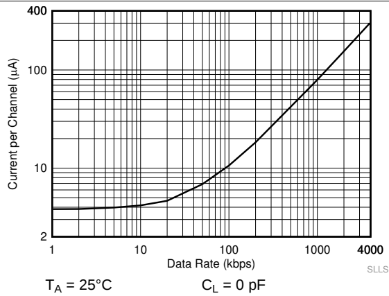
图 3. ISO7021 Supply Current vs Data Rate at 1.8 V (With No Load)
