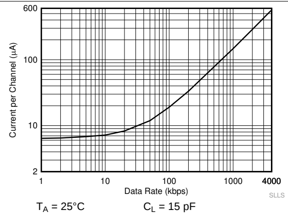
图 10. ISO7021 Supply Current vs Data Rate at 5 V (With 15-pF Load)
