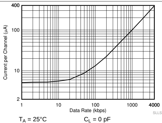
图 7. ISO7021 Supply Current vs Data Rate at 3.3 V (With No Load)
