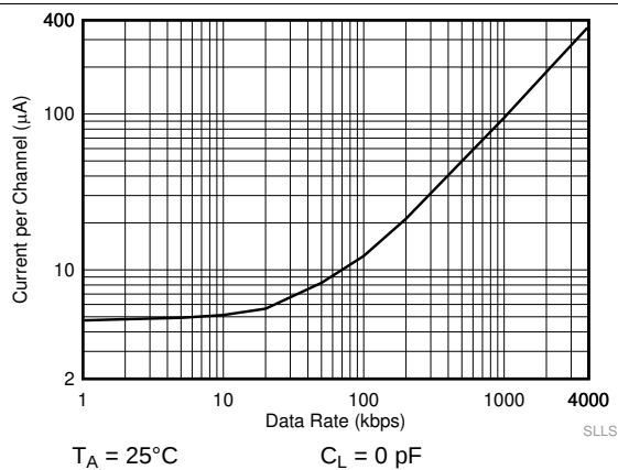
图 5. ISO7021 Supply Current vs Data Rate at 2.5 V (With No Load)
