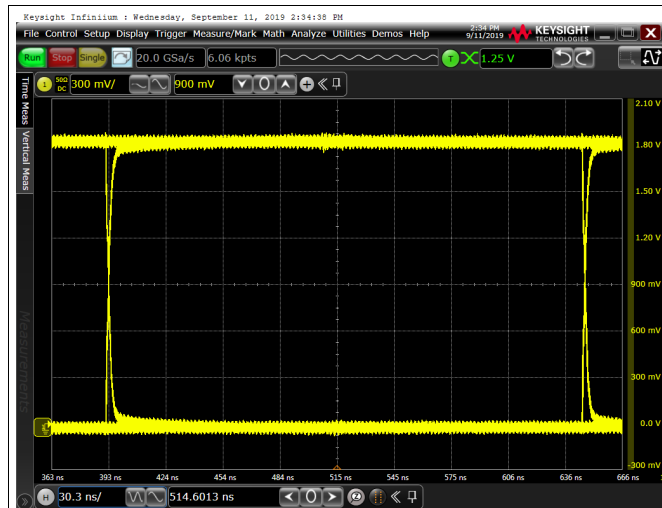
图 20. Eye Diagram at 4 Mbps PRBS 2^{16} - 1 , 1.8 V and 25°C
