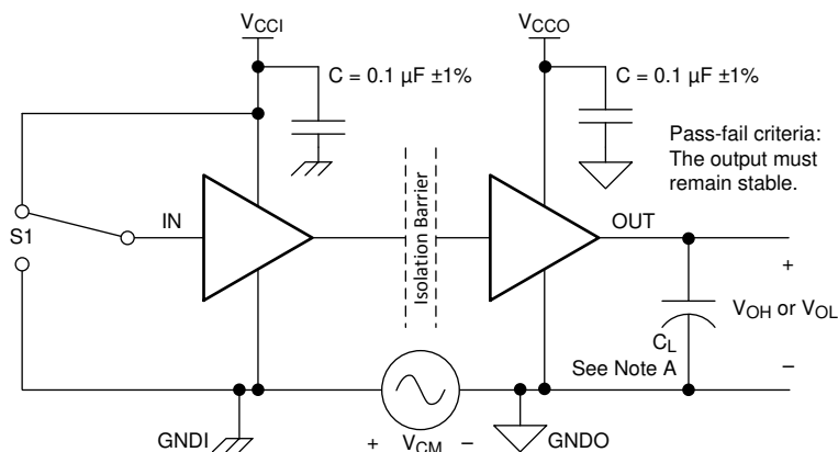
图 12. Default Output Delay Time Test Circuit and Voltage Waveforms
