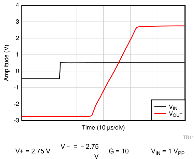
图 7-47. Over-Load Recovery (Rising Edge)
