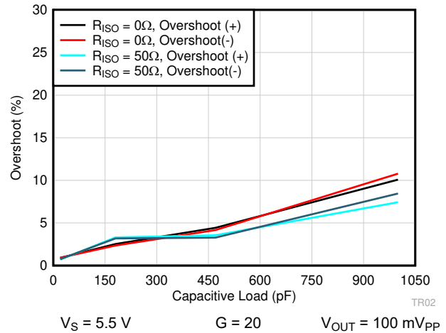
图 7-40. Small-Signal Overshoot vs Capacitive Load
