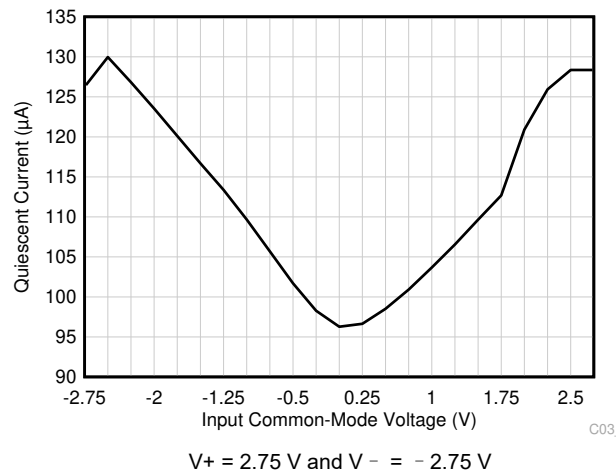
图 7-23. Quiescent Current vs Input Common-Mode Voltage
