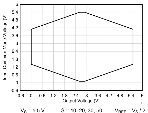
图 7-57. Input Common-Mode Voltage vs Output Voltage
