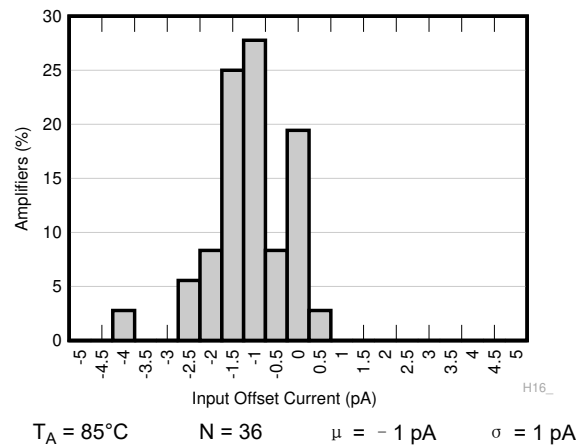
图 7-6. Typical Distribution of Input Offset Current
