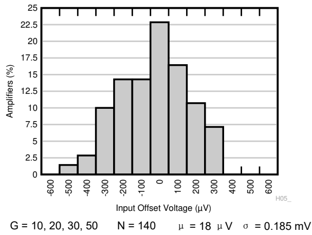
图 7-1. Typical Distribution of Input Referred Offset Voltage
