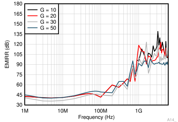
图 7-38. Electromagnetic Interference Rejection Ratio Referred to Noninverting Input (EMIRR+) vs Frequency
