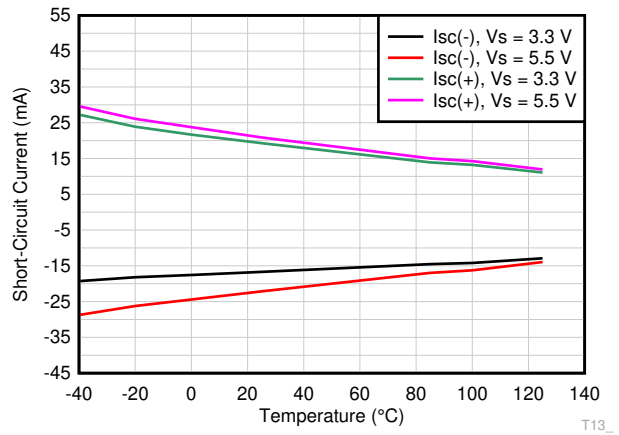
图 7-16. Short Circuit Current vs Temperature
