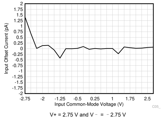
图 7-22. Input Offset Current vs Input Common-Mode Voltage
