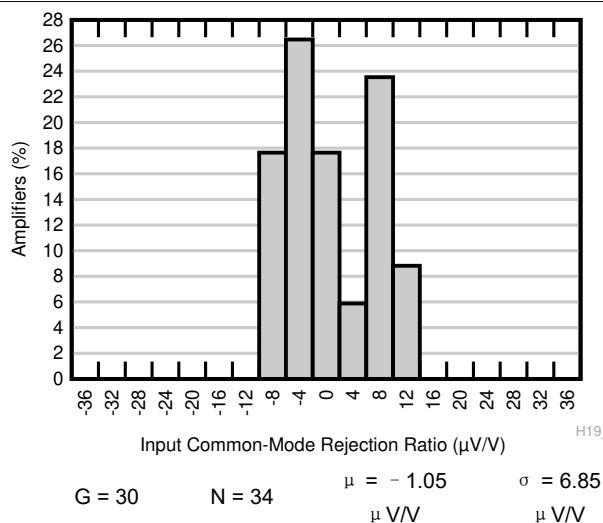
图 7-9. Typical Distribution of CMRR
