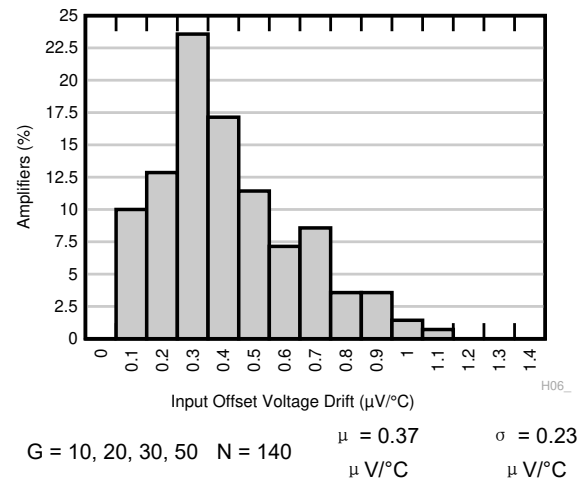
图 7-2. Typical Distribution of Input Referred Offset Drift
