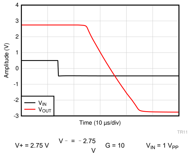
图 7-48. Over-Load Recovery (Falling Edge)
