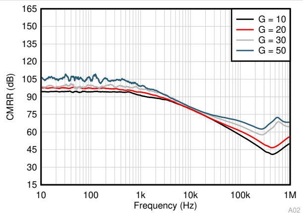
图 7-29. CMRR (Referred to Input) vs Frequency
