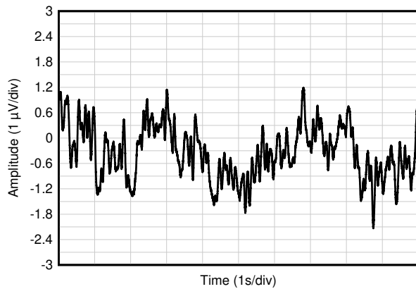
图 7-33. 0.1 Hz to 10 Hz Voltage Noise in Time Domain
