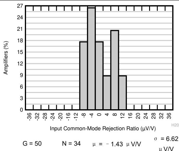
图 7-10. Typical Distribution of CMRR
