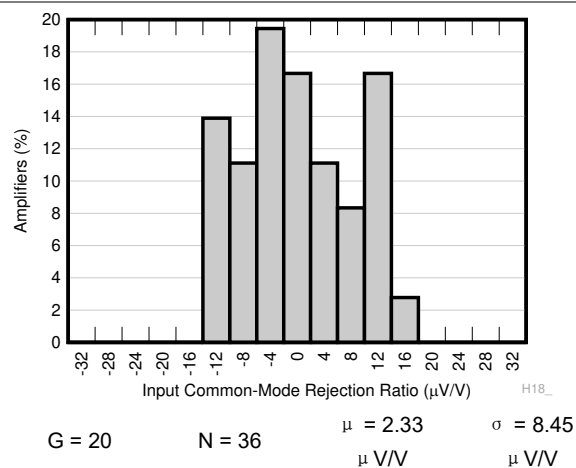
图 7-8. Typical Distribution of CMRR
