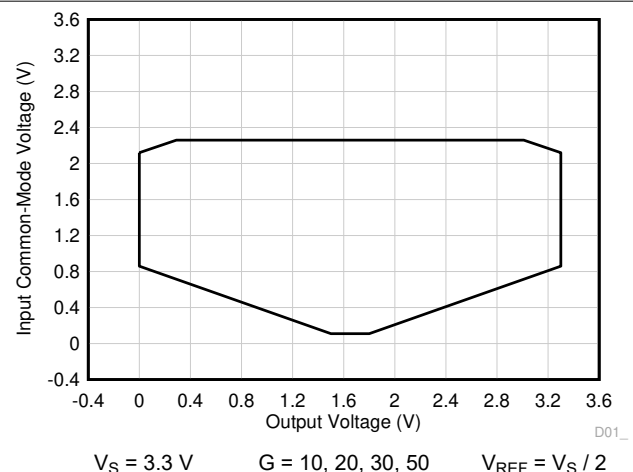
图 7-52. Input Common-Mode Voltage vs Output Voltage (High CMRR Region)
