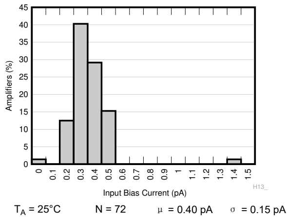
图 7-3. Typical Distribution of Input Bias Current
