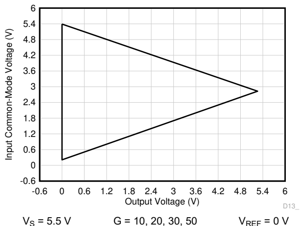
图 7-59. Input Common-Mode Voltage vs Output Voltage
