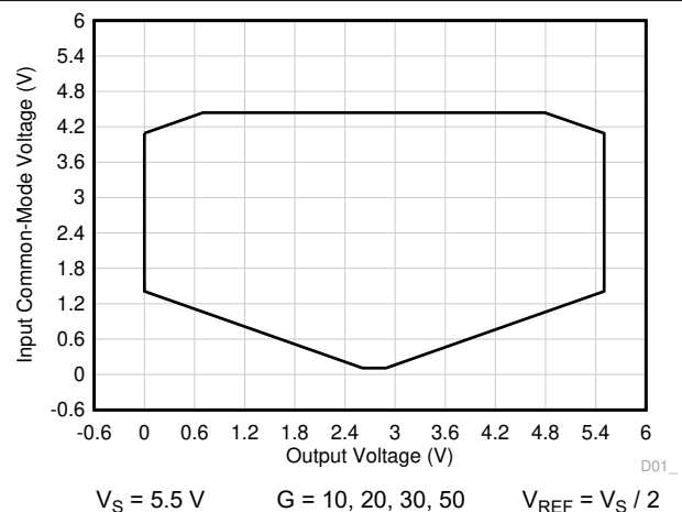
图 7-53. Input Common-Mode Voltage vs Output Voltage (High CMRR Region)
