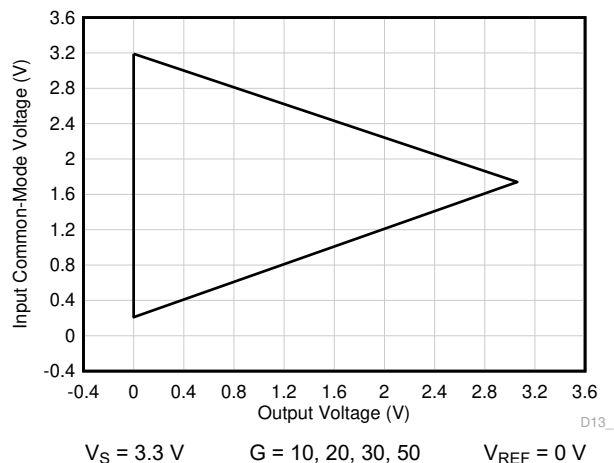
图 7-58. Input Common-Mode Voltage vs Output Voltage
