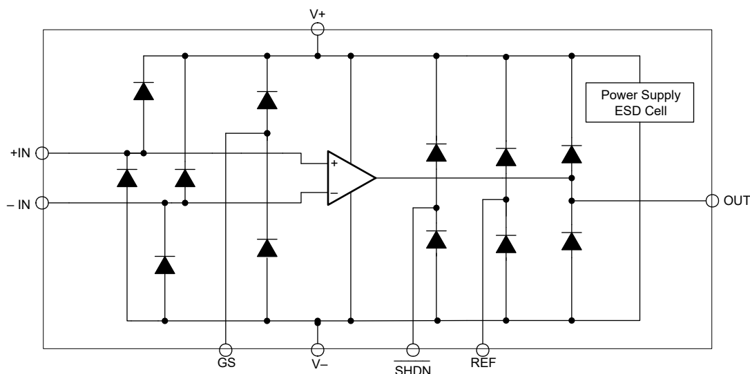
图 8-5. Equivalent Internal ESD Circuitry
