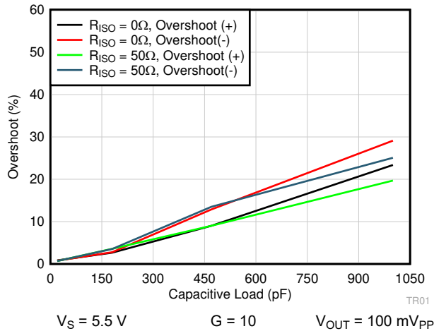
图 7-39. Small-Signal Overshoot vs Capacitive Load
