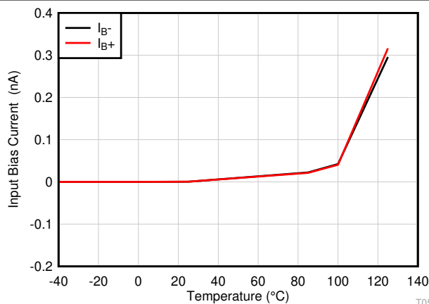
图 7-12. Input Bias Current vs Temperature
