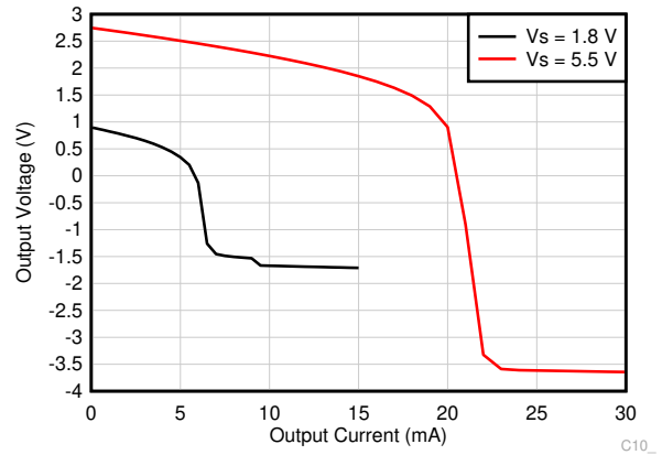
图 7-26. Output Voltage vs Output Current (Sourcing)
