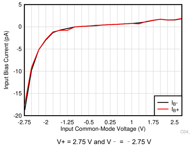
图 7-21. Input Bias Current vs Input Common-Mode Voltage
