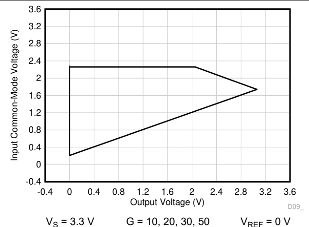
图 7-54. Input Common-Mode Voltage vs Output Voltage (High CMRR Region)
