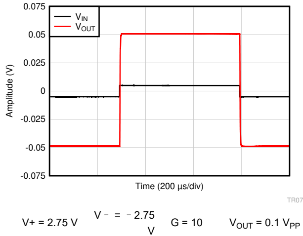
图 7-45. Small-Signal Step Response
