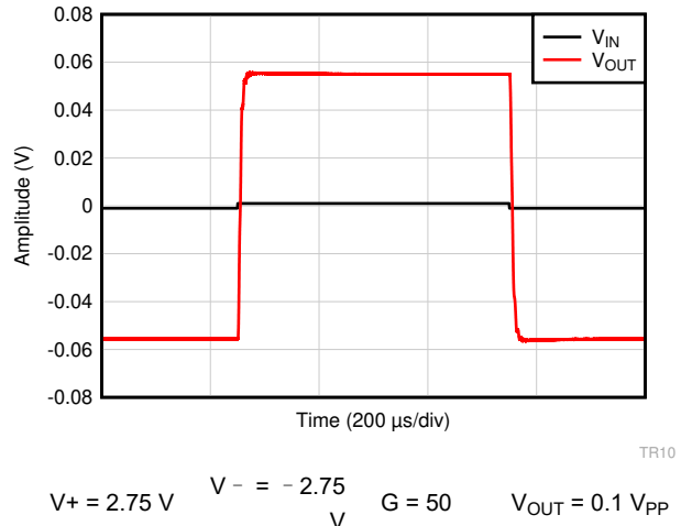
图 7-46. Small-Signal Step Response
