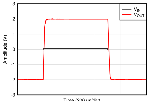
图 7-42. Large Signal Settling Time (Falling Edge)
