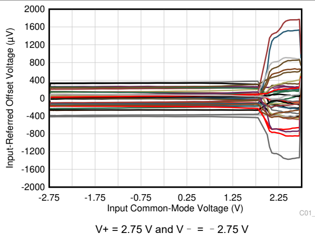
图 7-19. Input Referred Offset Voltage vs Input Common-Mode Voltage
