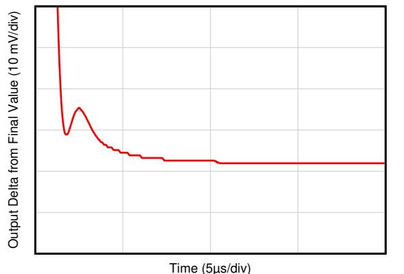
图 7-41. Large Signal Step Response
