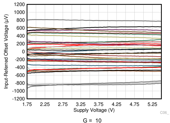
图 7-24. Input Referred Offset Voltage vs Supply Voltage
