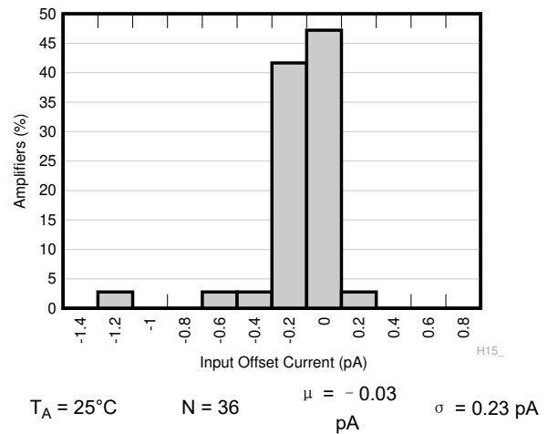
图 7-4. Typical Distribution of Input Offset Current
