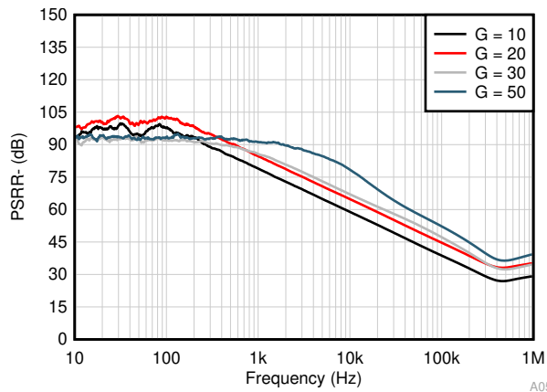
图 7-31. PSRR - (Referred to Input) Vs Frequency
