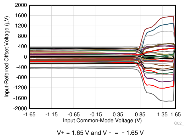
图 7-20. Input Referred Offset Voltage vs Input Common-Mode Voltage
