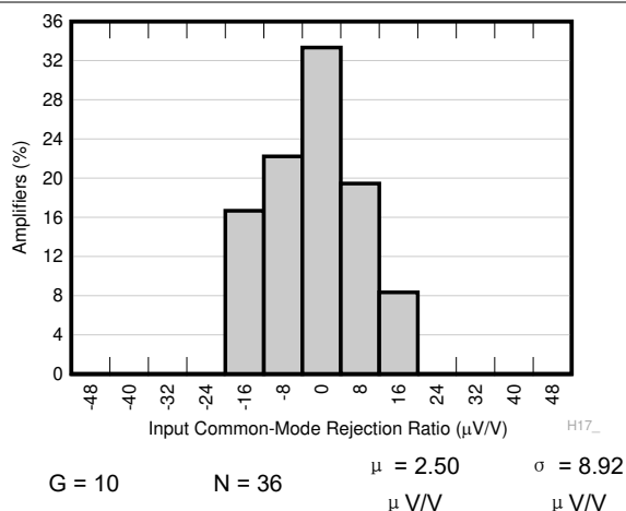
图 7-7. Typical Distribution of CMRR
