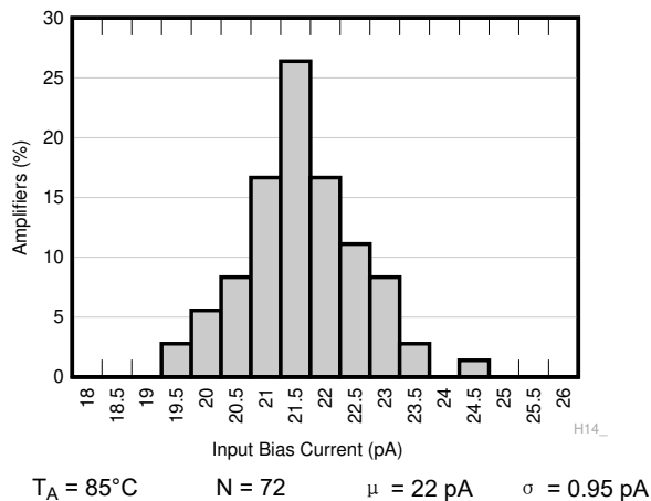
图 7-5. Typical Distribution of Input Bias Current
