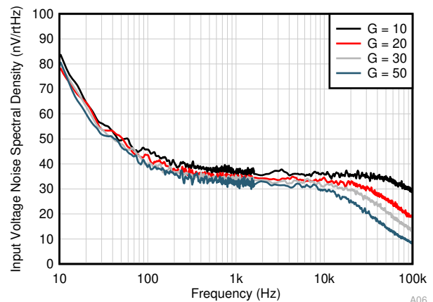
图 7-32. Input Referred Voltage Noise Spectral Density
