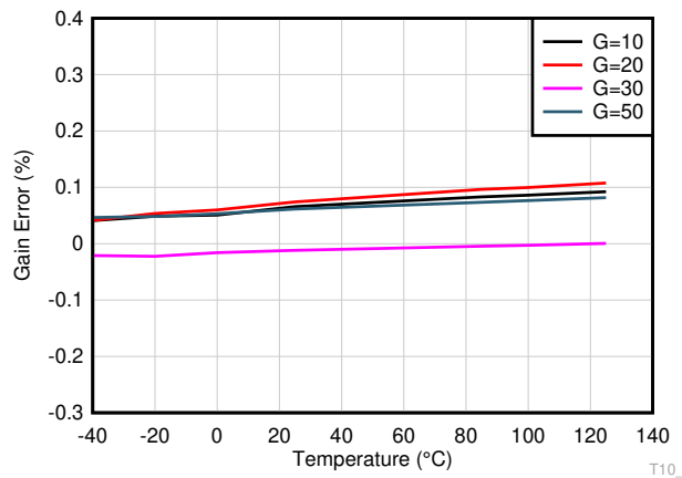
图 7-17. Gain Error vs Temperature
