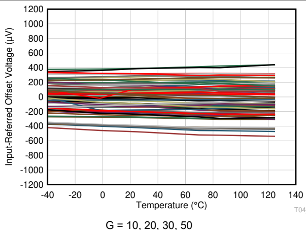
图 7-11. Input Referred Offset Voltage vs Temperature
