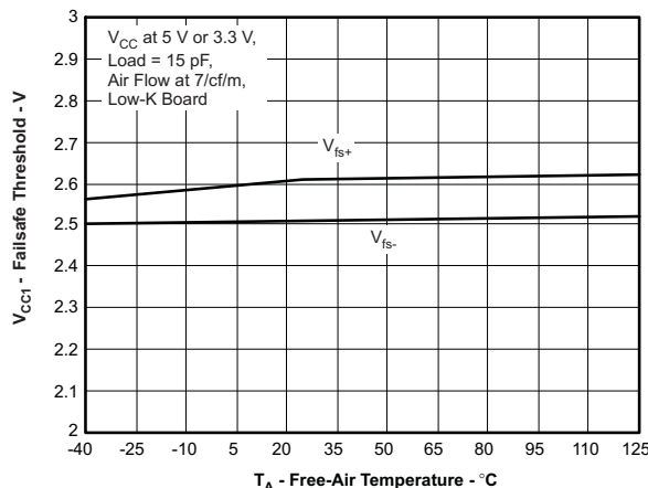
Figure 5. V_{CC1} Fail-Safe Threshold vs Free-Air Temperature
