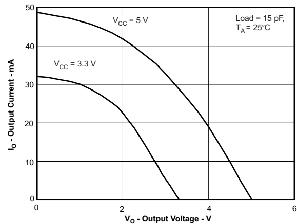
Figure 6. High-Level Output Current vs High-Level Output Voltage
