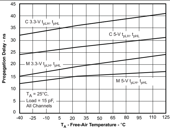
Figure 3. Propagation Delay vs Free-Air Temperature
