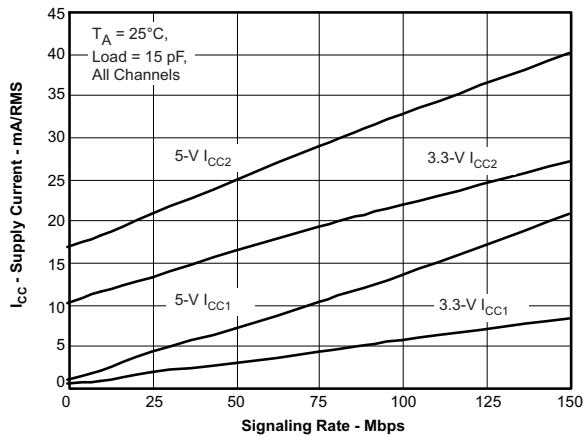
Figure 1. ISO7230C/M RMS Supply Current vs Signaling Rate
