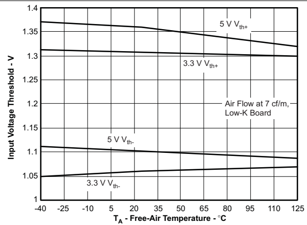
Figure 4. Input Threshold Voltage vs Free-Air Temperature
