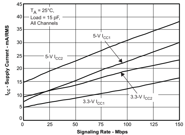
Figure 2. ISO7231C/M RMS Supply Current vs Signaling Rate
