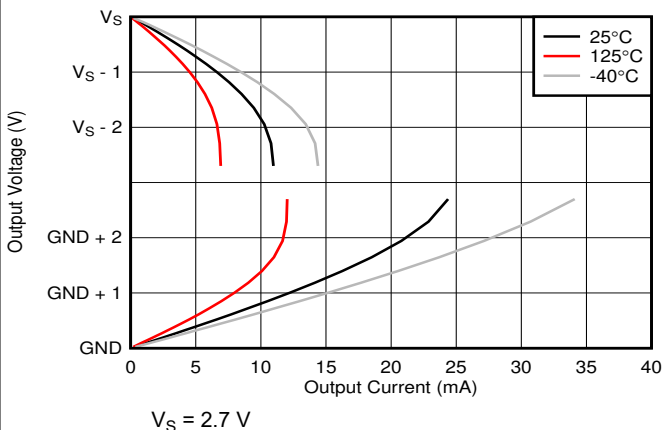
图 6-18. Output Voltage vs Output Current
