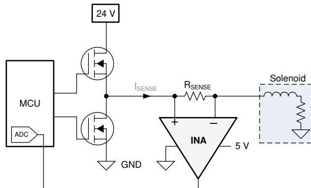
图 8-2. Current Sensing in a Solenoid Application
