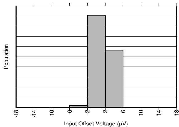
图 6-5. INA293x5 Input Offset Production Distribution
