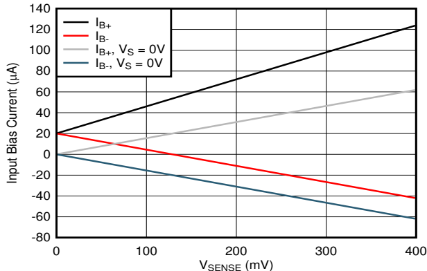
图 6-16. INA293x2Q, INA293x3Q Input Bias Current vs V_{\text{SENSE}}
