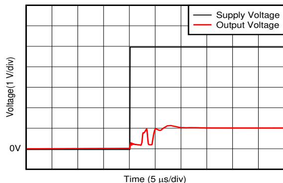
图 6-33. Start-Up Response
