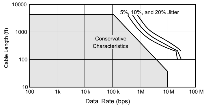
图 53. Cable Length vs Data Rate Characteristics
