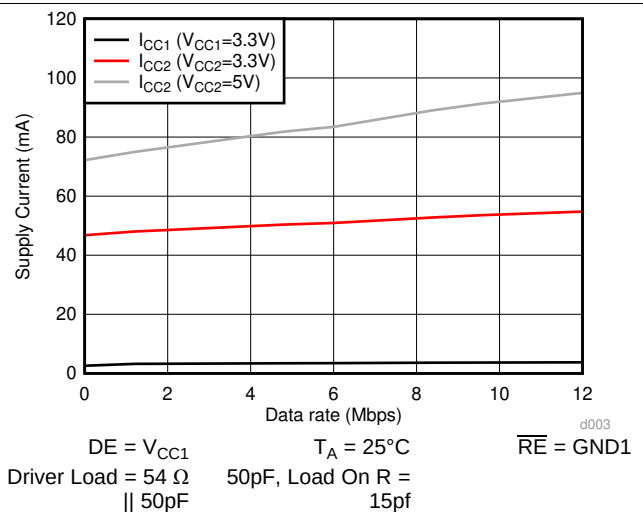
图 8. ISO143x Supply Current Vs Data Rate- 54Ω||50pF Load
