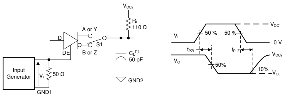
图 41. Driver Enable and Disable Times
