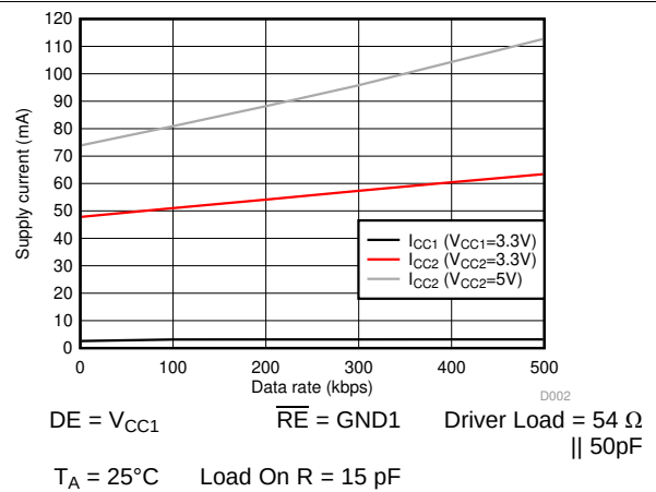
图 4. ISO141x Supply Current Vs Data Rate- With 54Ω||50pF Load
