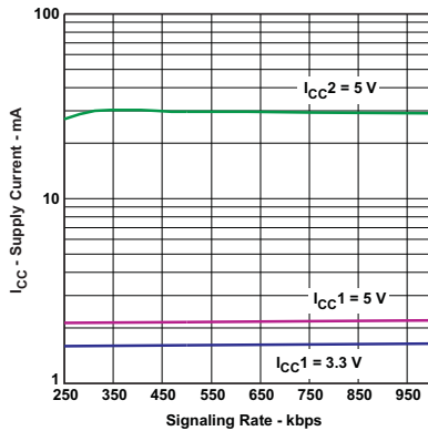
图 3. Supply Current (RMS) vs Signaling Rate (kbps)
