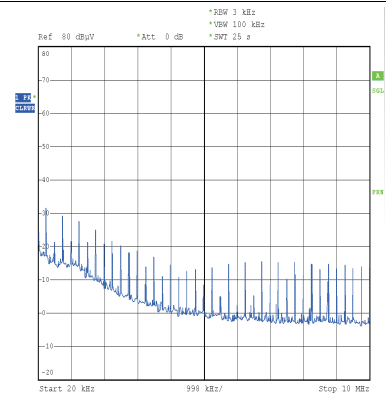
图 5. Emissions Spectrum to 10 MHz
