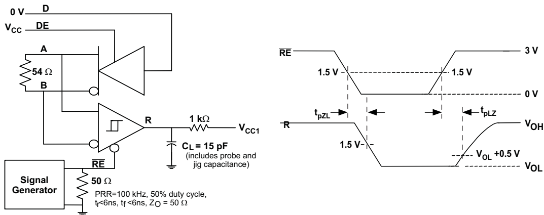
Figure 25. Receiver Enable Test Circuit and Waveforms, Data Output Low
