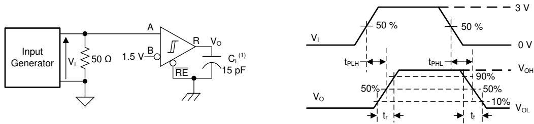
图 42. Receiver Switching Specifications
