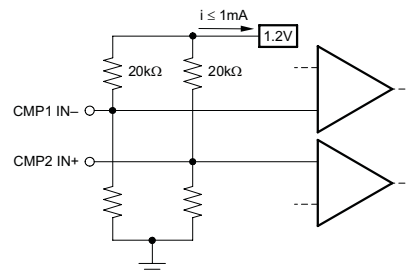
Figure 33. Limit Current Into Reference \leq 1 \text{ mA}
