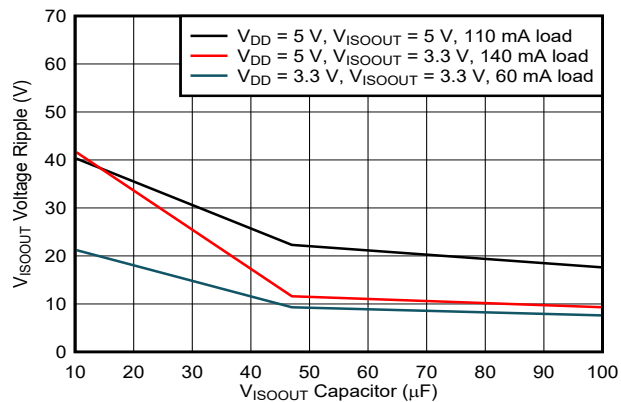
图 7-28. V_{ISOOUT} Ripple Voltage vs Load Capacitor
