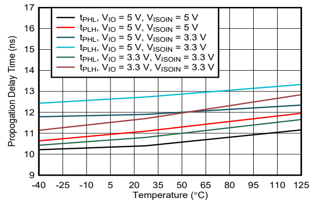
图 7-14. Propagation Delay Time vs Free-Air Temperature
