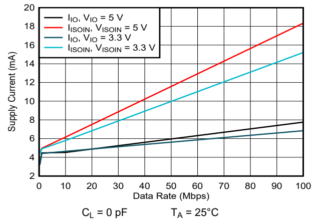
图 7-12. ISOW7741 Channel Supply Currents vs Data Rate For C_L = 0\text{ pF}
