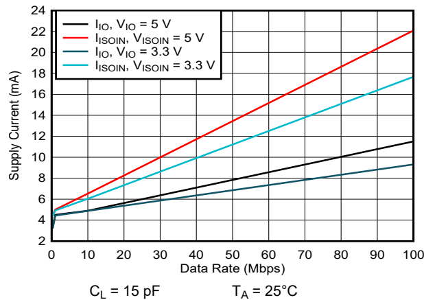
图 7-11. ISOW7741 Channel Supply Currents vs Data Rate For C_L = 15\text{ pF}
