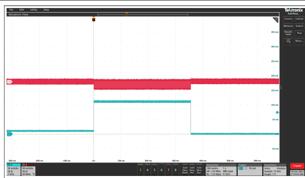
图 7-17. 10-mA to 110-mA Load Transient Response
