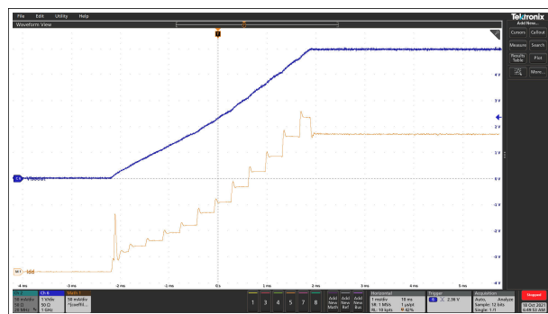
图 7-29. Soft Start at 10-mA Load For V_{ISOOUT} = 5\text{ V}
