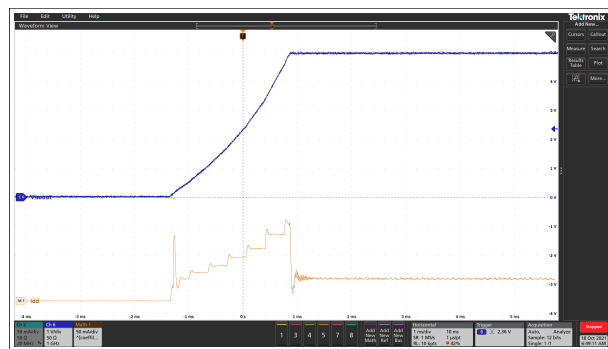
图 7-27. Soft Start at 50-mA Load For V_{ISOOUT} = 3.3\text{ V}
