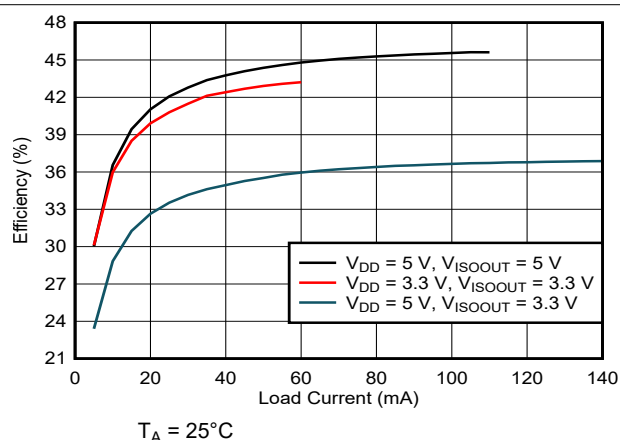
图 7-6. Efficiency vs Load Current ( I_{ISOOUT} )
