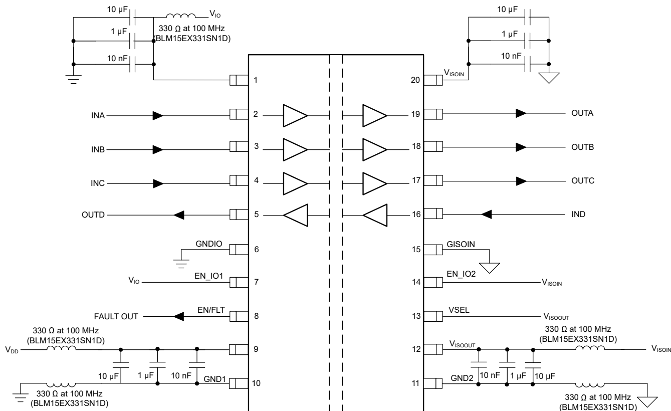
图 10-2. Typical ISOW7741 Circuit Hook-Up
