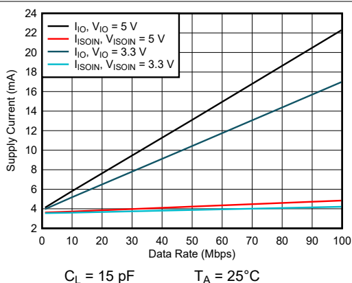
图 7-19. ISOW7744 Channel Supply Currents vs Data Rate For C_L = 15 \text{ pF}
