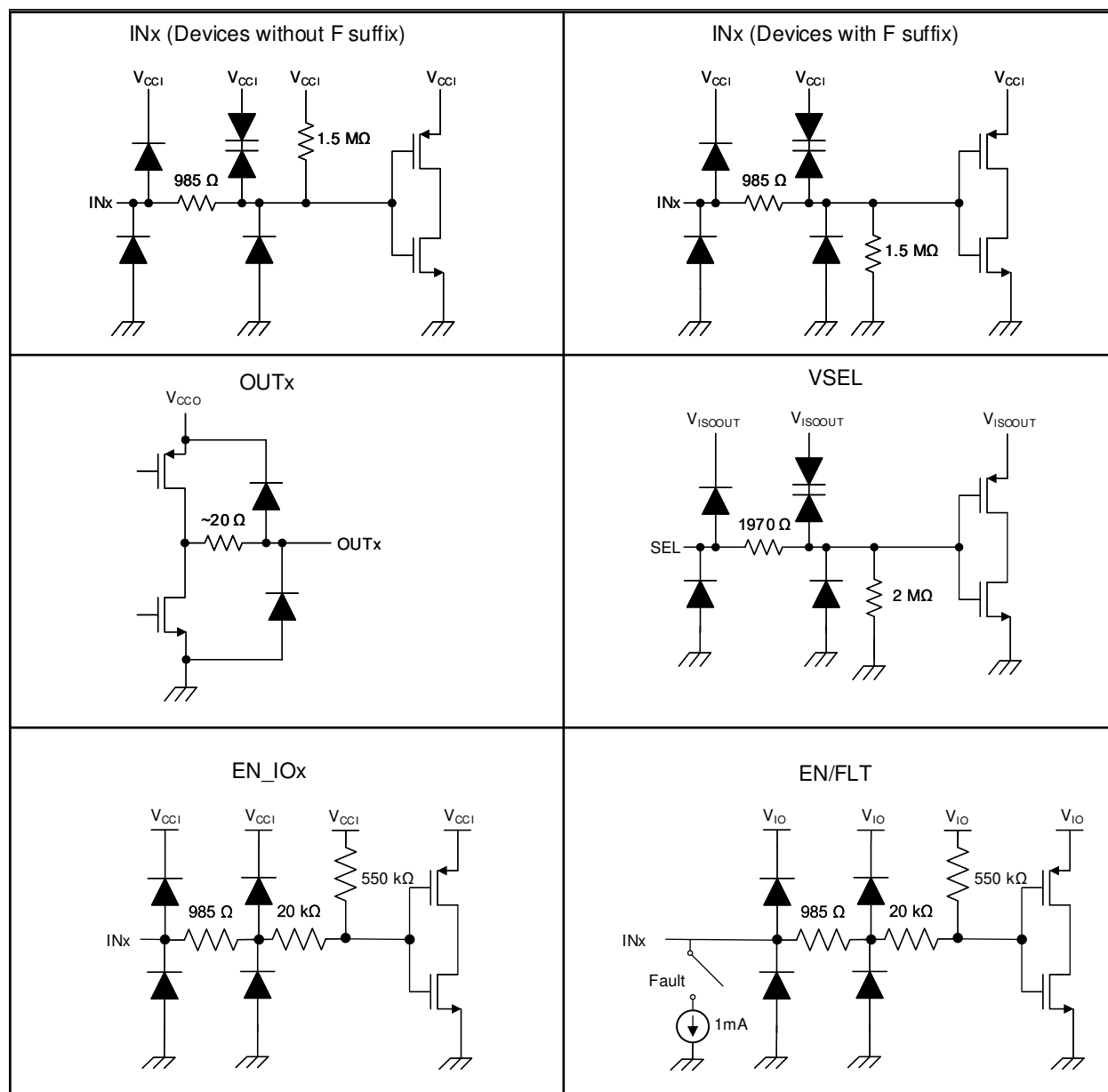
图 9-5. Device I/O Schematics
