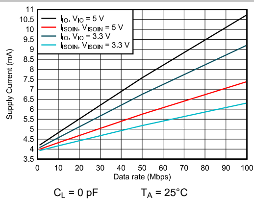
图 7-18. ISOW7743 Channel Supply Currents vs Data Rate For C_L = 0 \text{ pF}
