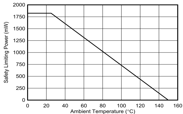
图 7-2. Thermal Derating Curve for Safety Limiting Power for DFM-20 Package
