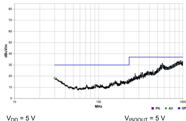
图 10-3. ISOW7741 Radiated Emissions versus CISPR32B line (Blue)
