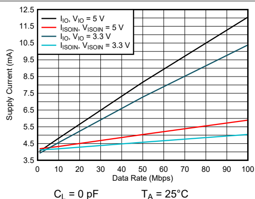
图 7-20. ISOW7744 Channel Supply Currents vs Data Rate For C_L = 0 \text{ pF}
