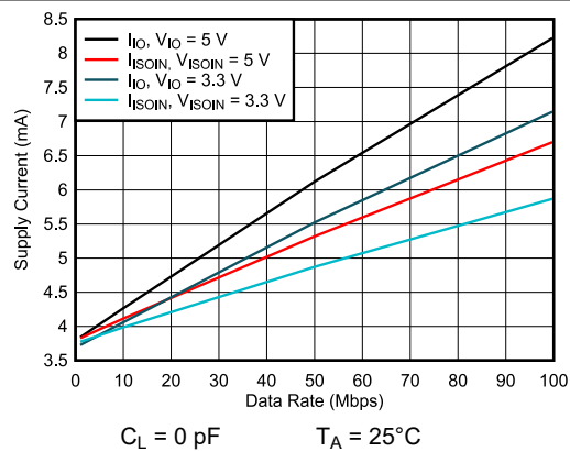
图 7-16. ISOW7742 Channel Supply Currents vs Data Rate For C_L = 0 \text{ pF}
