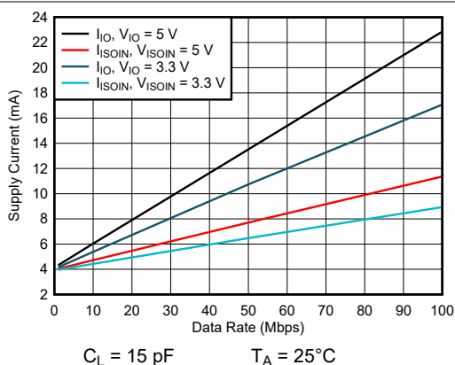
图 7-17. ISOW7743 Channel Supply Currents vs Data Rate For C_L = 15 \text{ pF}
