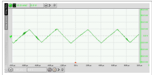
V_{DD} = 3.3\text{ V} V_{ISOOUT} = 3.3\text{ V} 10 uF V Capacitor on V_{ISOOUT}
