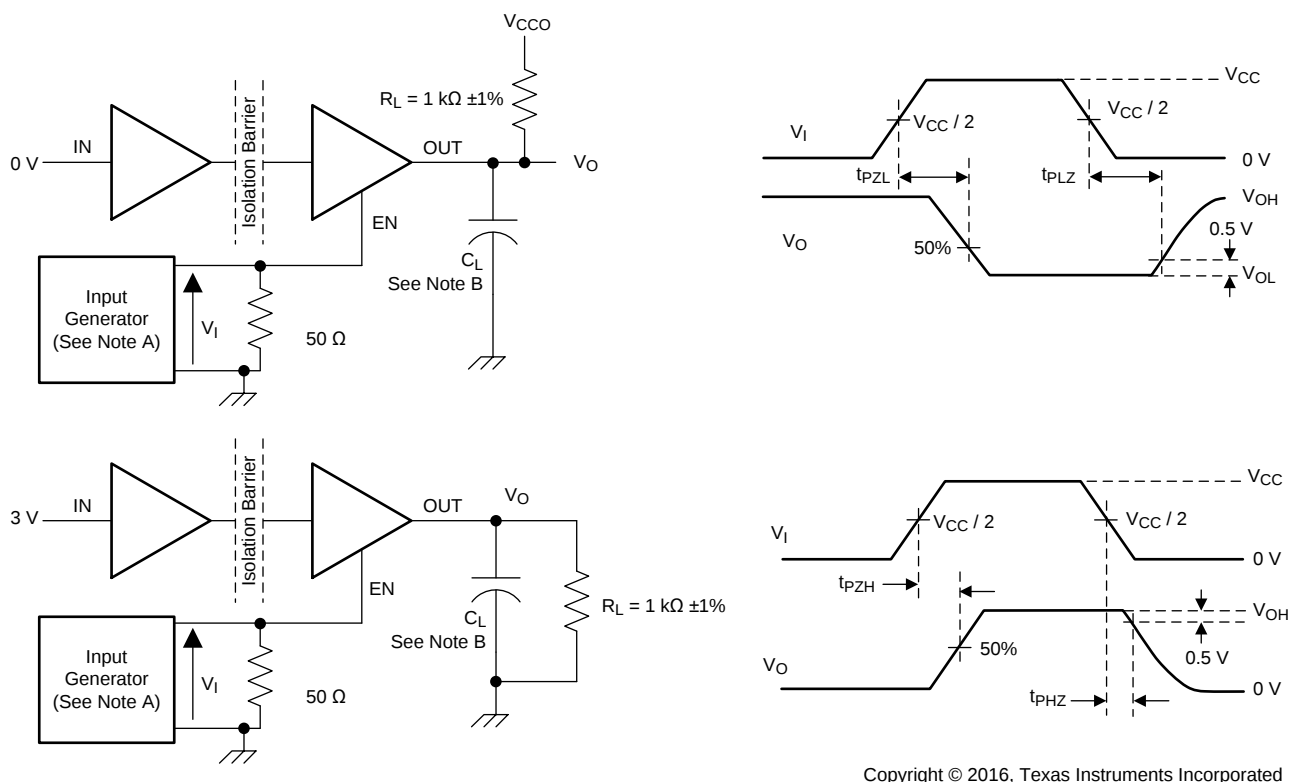
Figure 15. Switching Characteristics Test Circuit and Voltage Waveforms
