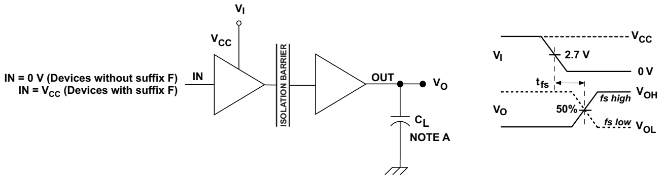
Figure 12. Fail-Safe Output Delay-Time Test Circuit and Voltage Waveforms
