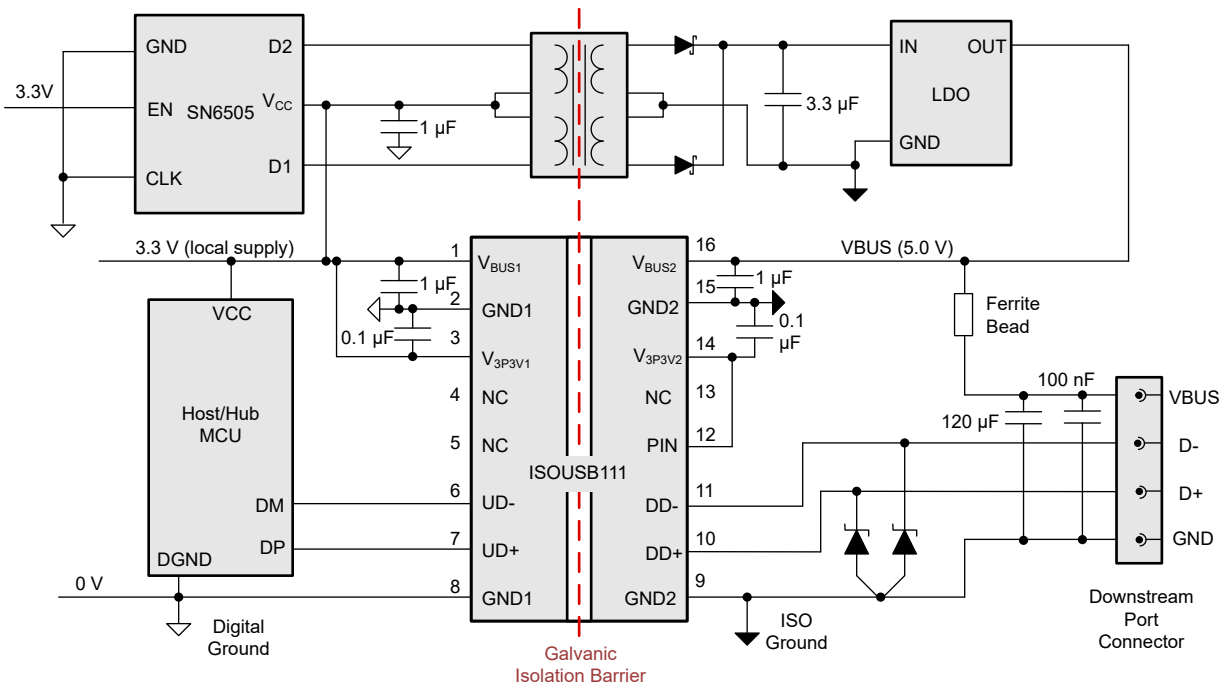
图 10-1. Isolated Host or Hub with ISOUSB111
