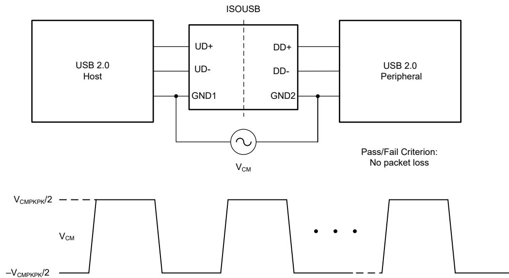
图 7-2. Common-Mode Transient Immunity Test Circuit
