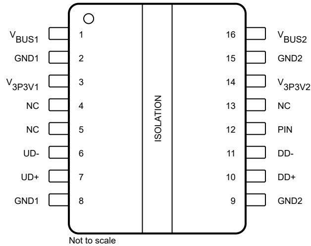
图 5-1. DW Package 16-Pin SOIC Top View
