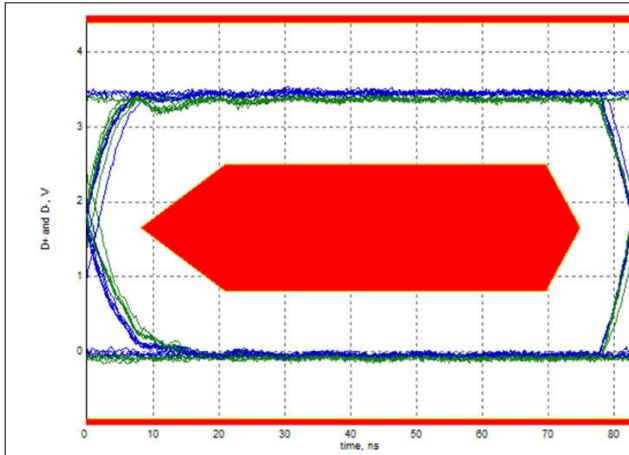
图 6-5. Typical Full-Speed (12 Mbps) Eye-Diagram through ISOUSB111
