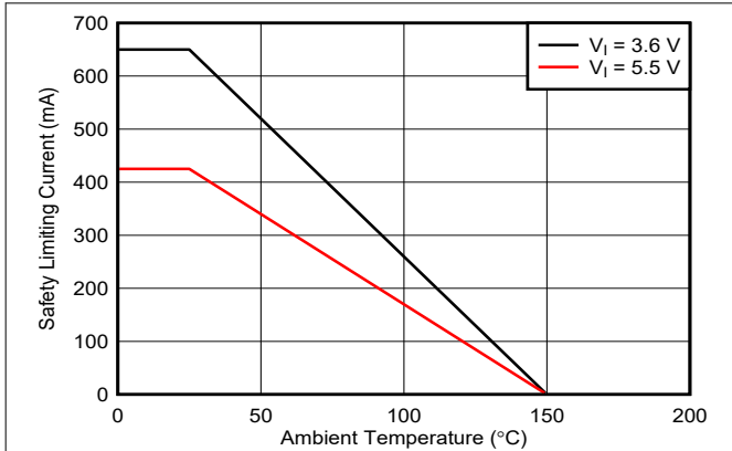
Figure 6-1. Thermal Derating Curve for Limiting Current per VDE for DW-16 Package
