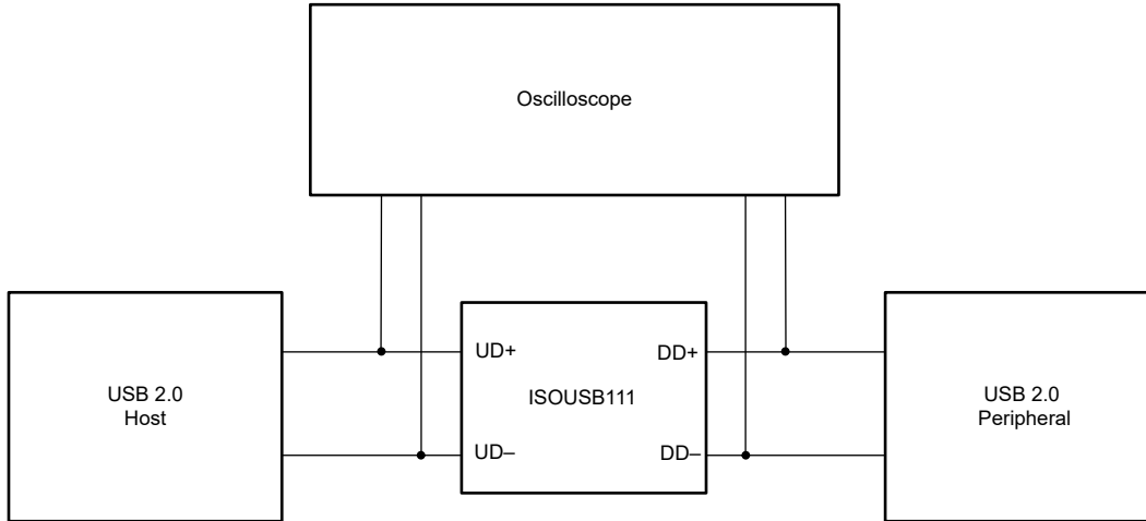
图 7-1. Upstream and Downstream Packet Parameter and Eye-Diagram Measurements
