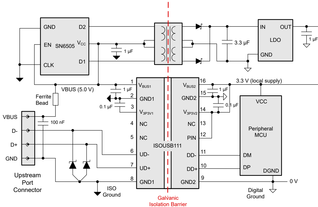
图 10-3. Isolated Bus-Powered Peripheral using ISOUSB111
