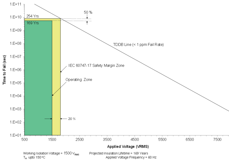
图 10-5. Insulation Lifetime Projection Data
