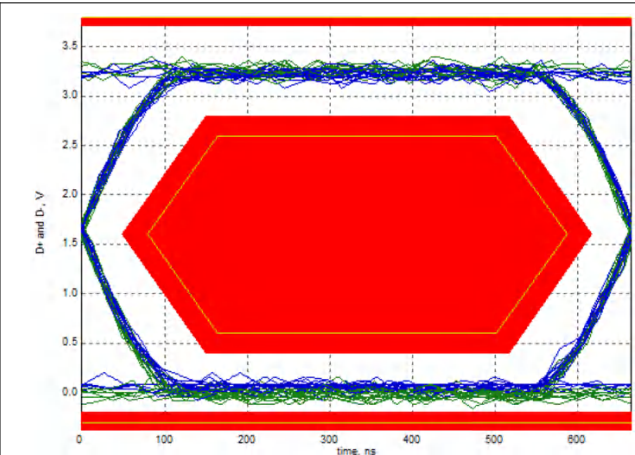
图 6-6. Typical Low-Speed (1.5 Mbps) Eye-Diagram through ISOUSB111
