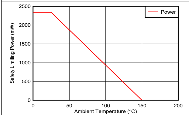
Figure 6-3. Thermal Derating Curve for Limiting Power per VDE for DW-16 Package
