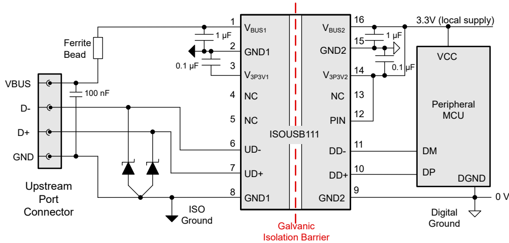
图 10-2. Isolated Self-Powered Peripheral with ISOUSB111
