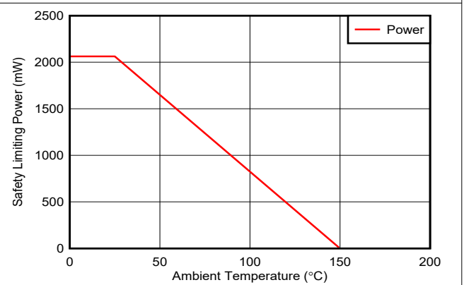
Figure 6-4. Thermal Derating Curve for Limiting Power per VDE for DWX-16 Package
