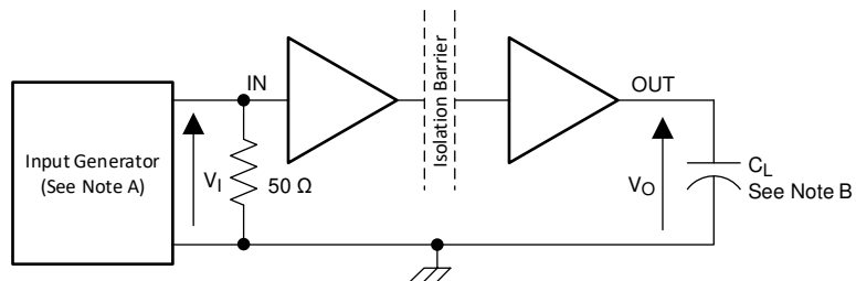
图 9-10. Short-Circuit Current Limiting
