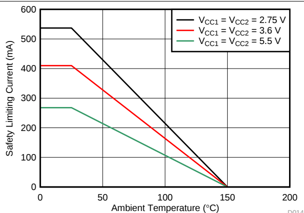
Figure 12. Thermal Derating Curve per VDE for DW-16 Package
