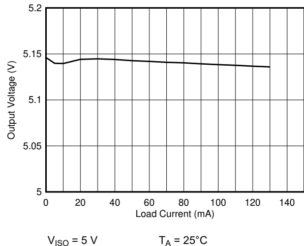
Figure 7-4. Isolated Supply Voltage ( V_{ISO} ) vs Load Current ( I_{ISO} )
