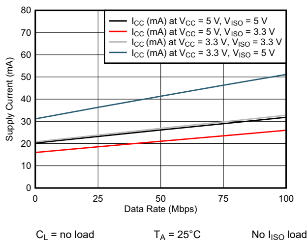
Figure 7-12. ISOW7841A-Q1 Supply Current vs Data Rate
