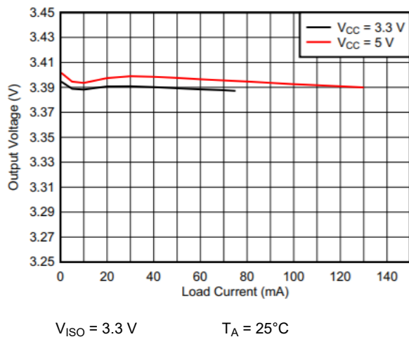
Figure 7-3. Isolated Supply Voltage ( V_{ISO} ) vs Load Current ( I_{ISO} )
