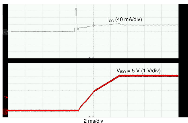
Figure 7-18. Soft Start at 10-mA Load
