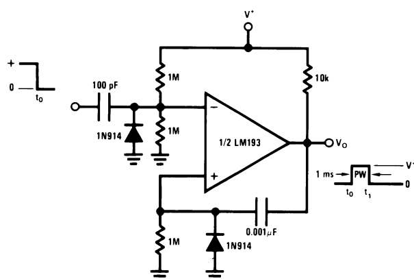
One-Shot Multivibrator
