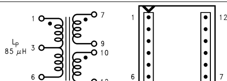
Figure 40. Renco RL-5534 (Top View)
