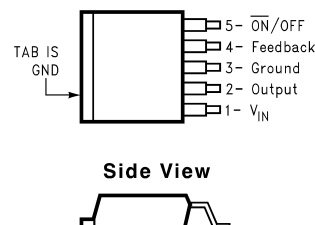
Figure 5-3. DDPK/TO-263 (S) Package 5-Lead Surface-Mount Package Top View
