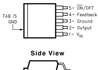
Figure 5-2. KTT Package 5-PIN DDPK/TO-263 Top View
