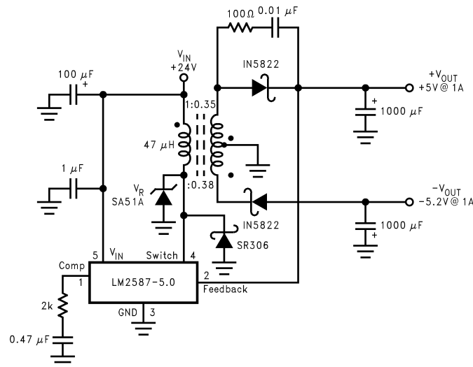
Figure 59. Flyback Regulator
