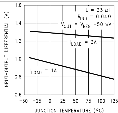
Figure 6. Dropout Voltage
