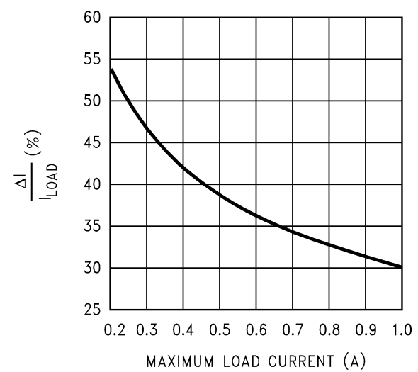
Figure 34. LM2590HV 5-V
