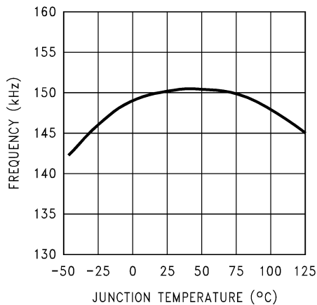
图 7-12. Switching Frequency
