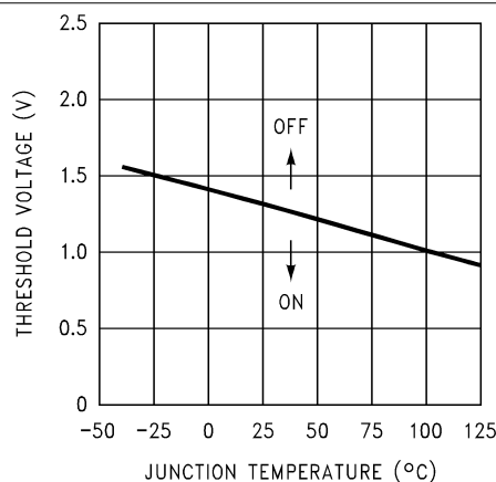
图 7-10. \overline{ON/OFF} Threshold Voltage
