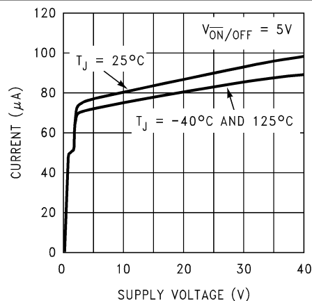
图 7-8. Shutdown Quiescent Current
