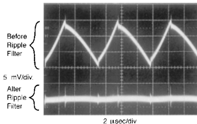
图 8-9. Post Ripple Filter Waveform
