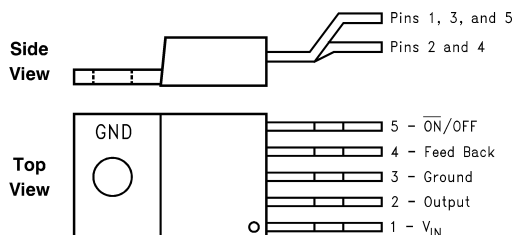
图 6-1. 5-Pin TO-220 NDH Package Top View
