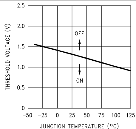
图 7-10. \overline{\text{ON/OFF}} Threshold Voltage
