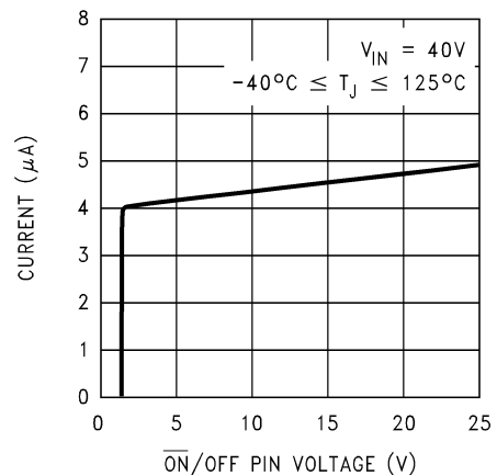
图 7-11. \overline{\text{ON/OFF}} Pin Current (Sinking)
