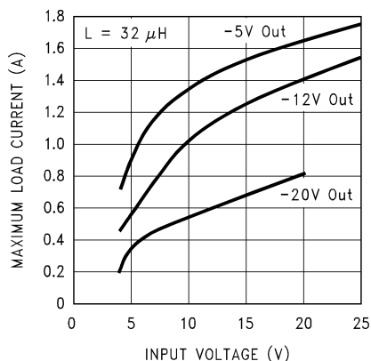
图 8-6. Inverting Regulator Typical Load Current
